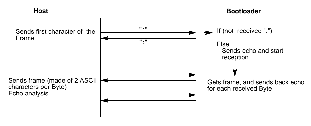
Figure 3. Command Flow
